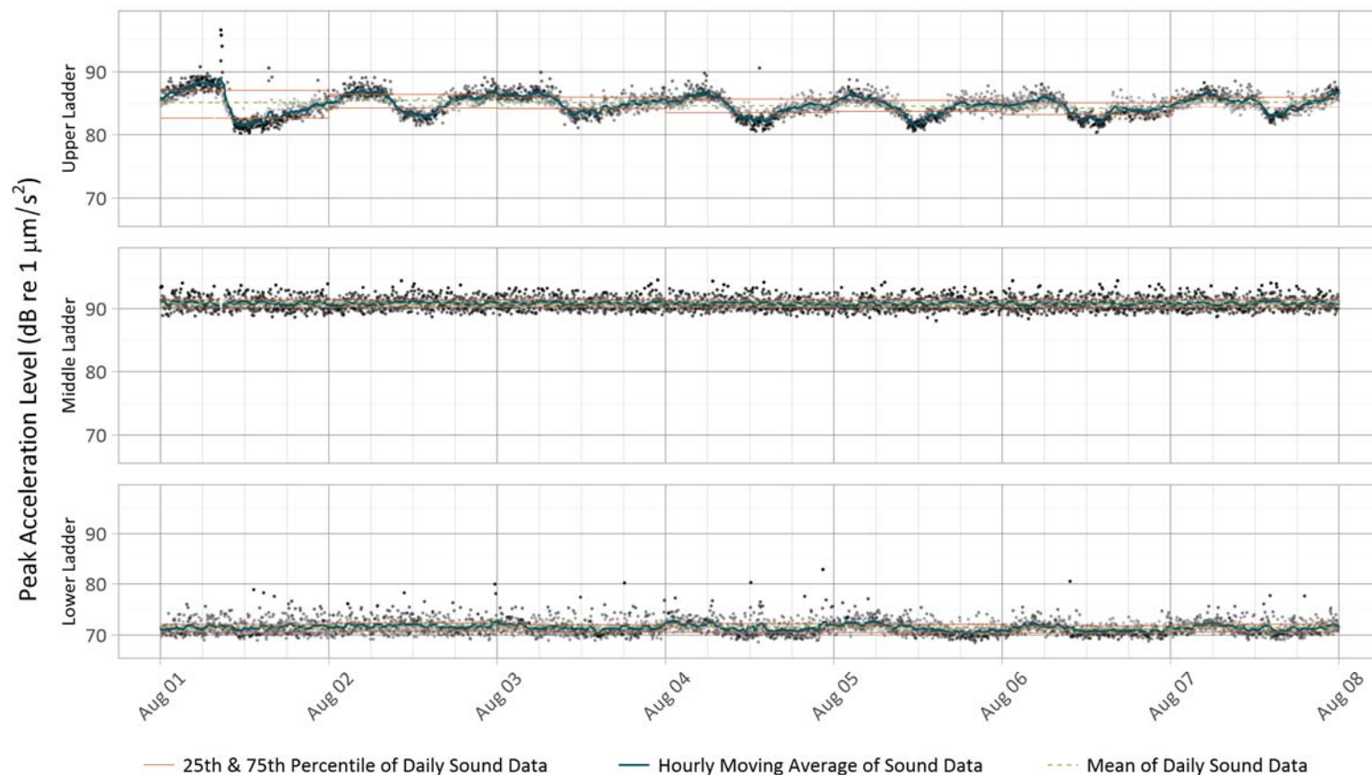
Figure 1 Peak Acceleration Levels Measured by Triaxial Accelerometers for Week 31
