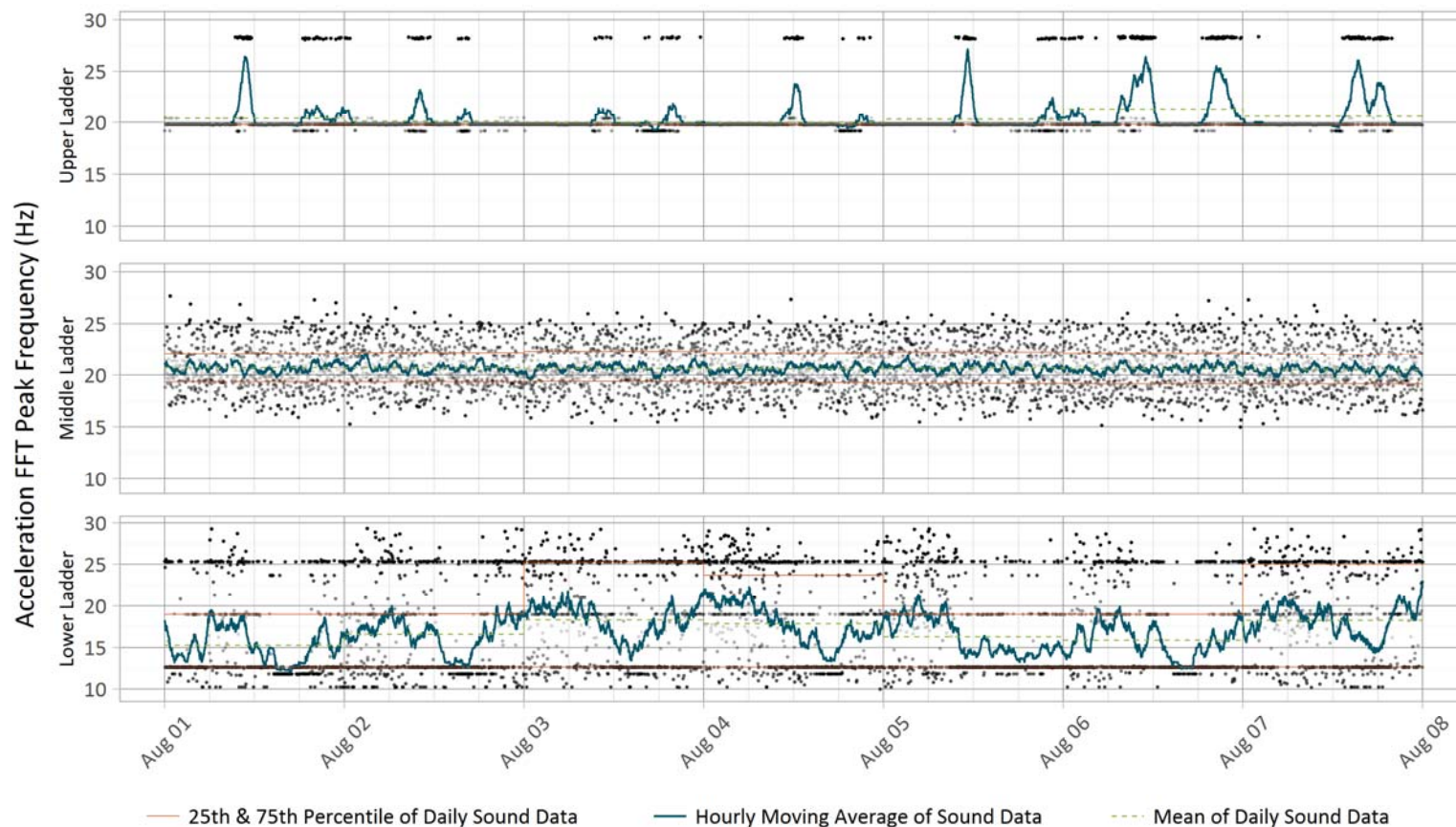
Figure 2 Acceleration Peak Frequencies Measured by Triaxial Accelerometers for Week 31
